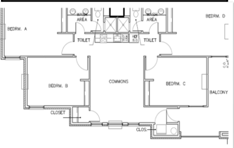
Apartment Building E, F and G Floor Plan
