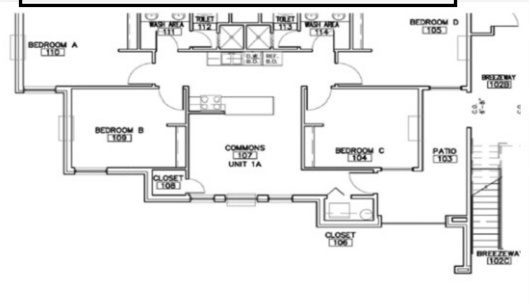
Apartment Building B Floor Plan
